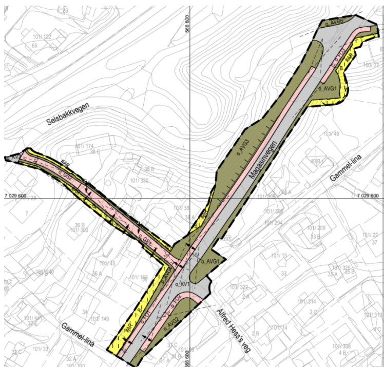
Figur 1 Plankart
